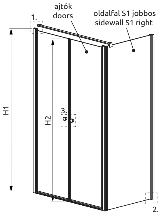
Balos kabin Variant L
