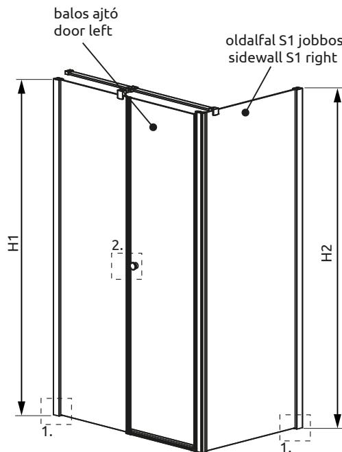
Balos kabin Variant L
